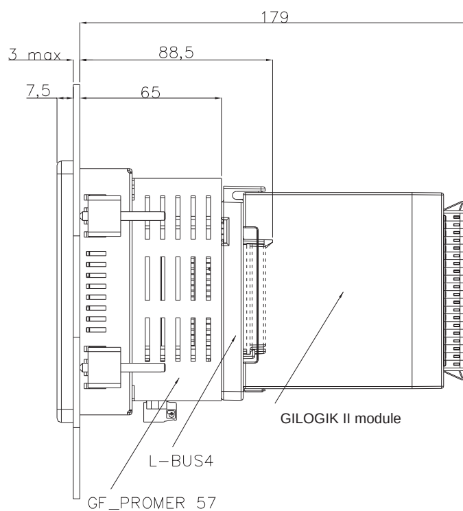
Overall dimensions - 57CT -
