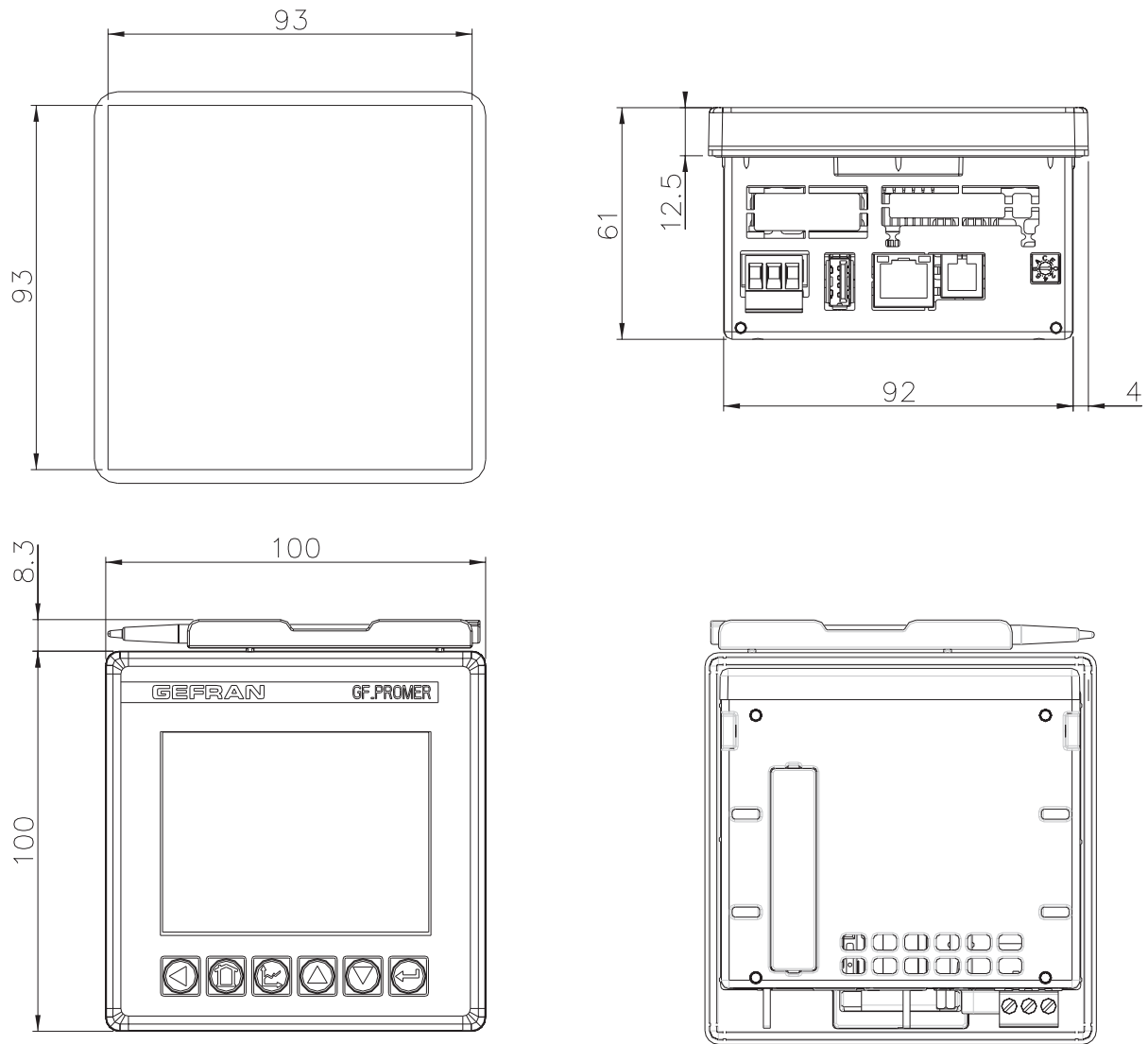
Physical dimensions and for drilling template - 35CT -
